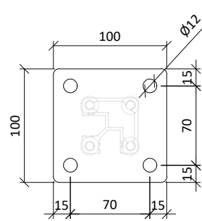
Corner Post Base Detail
