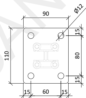
Mid Post Base Detail
