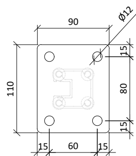
End Post Base Detail
