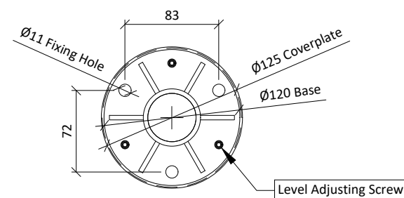
Ø120mm Baseplate Variant
