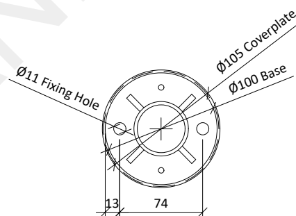
Ø100mm Baseplate Variant
