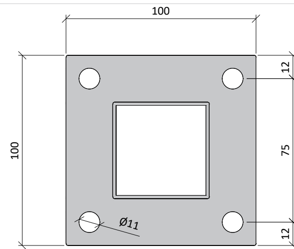
Baseplate Detail
