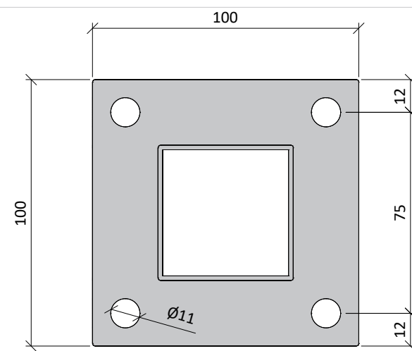
Baseplate Detail
